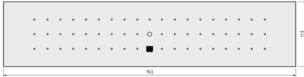
01 TOP VIEW
