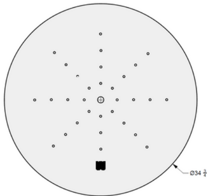
01 TOP VIEW
