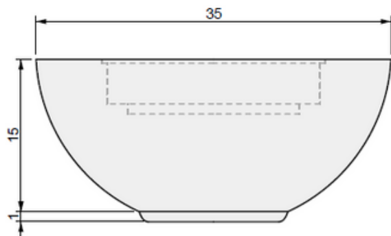
03 SIDE VIEW
