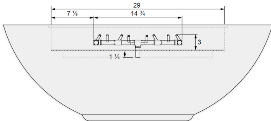
01 SIDE VIEW
