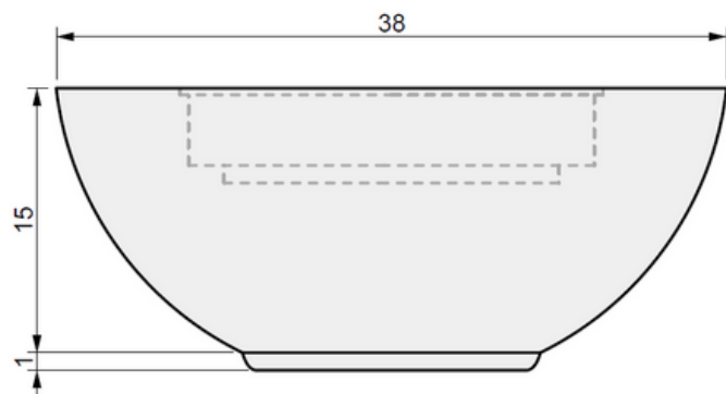
03 SIDE VIEW
