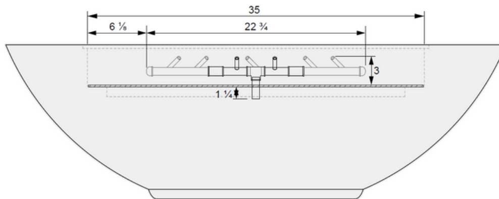
01 SIDE VIEW
