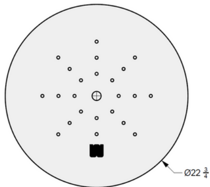
01 TOP VIEW
