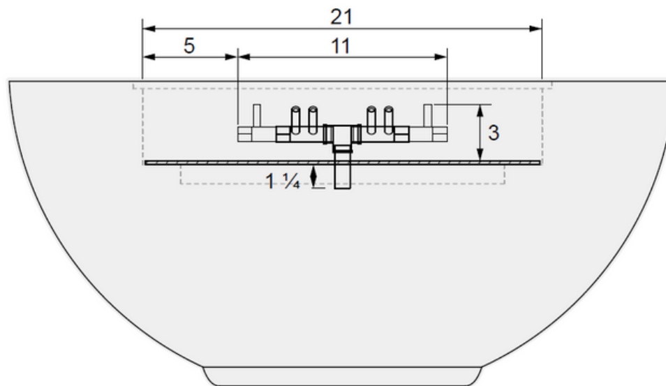
01 SIDE VIEW
