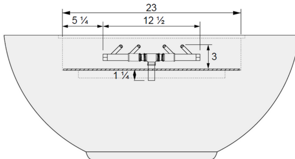
01 SIDE VIEW
