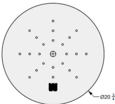
01 TOP VIEW
