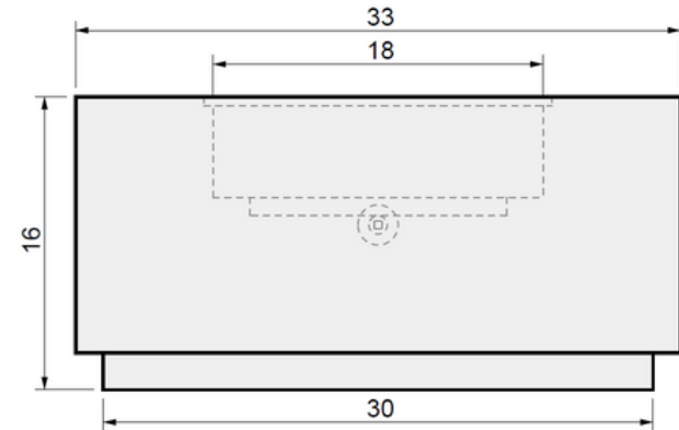
03 SIDE VIEW
