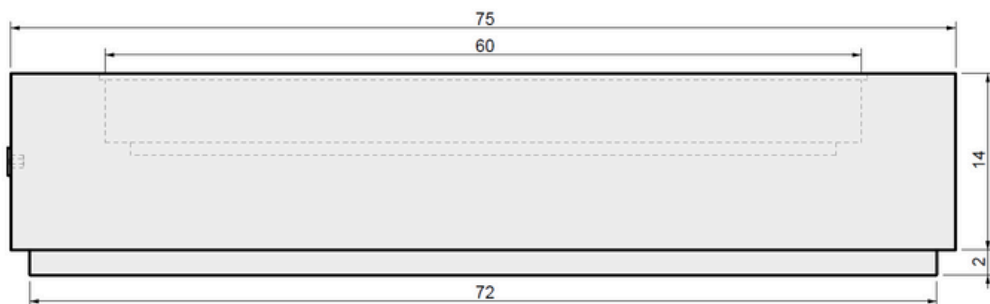
02 FRONT VIEW
