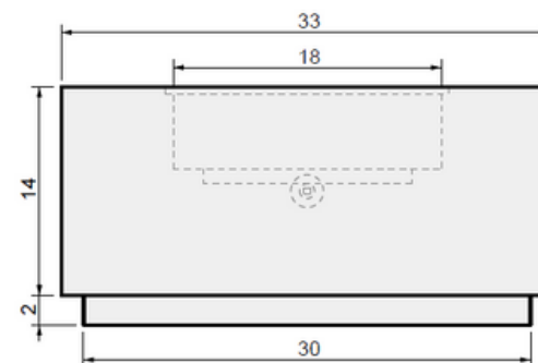
03 SIDE VIEW
