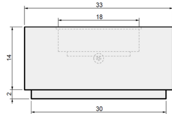
03 SIDE VIEW
