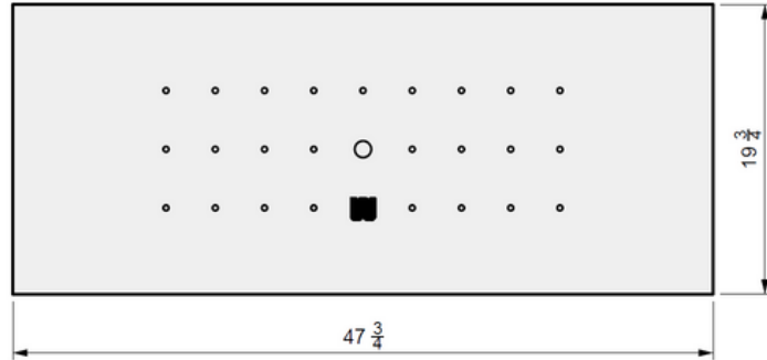
01 TOP VIEW
