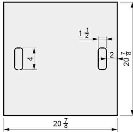
01 TOP VIEW
