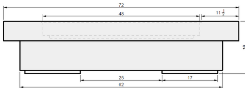
02 FRONT VIEW
