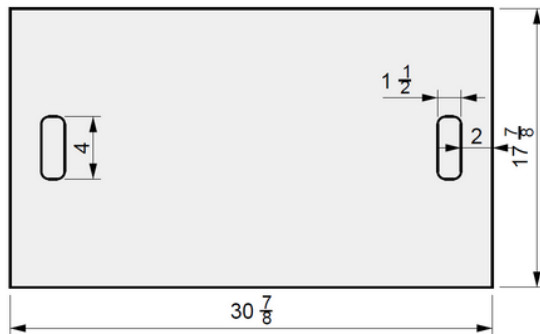
01 TOP VIEW
