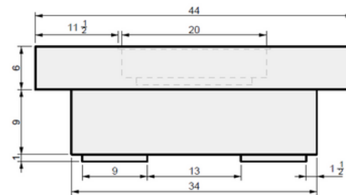
03 SIDE VIEW
